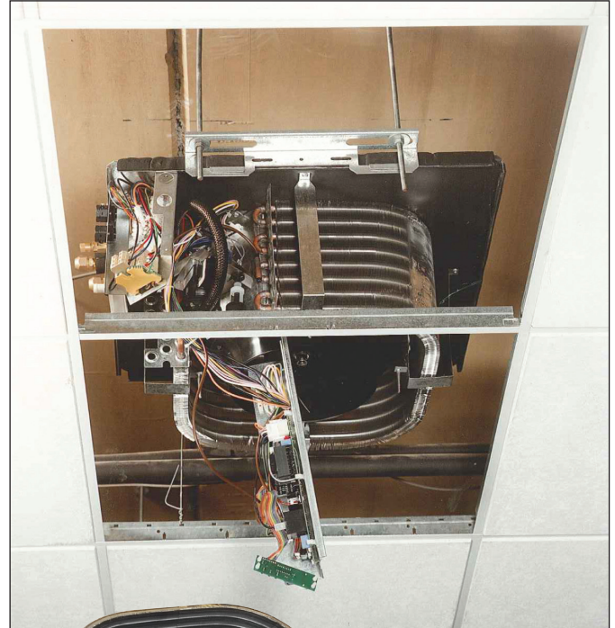
Single Diameter Fan (CC600) All services at one corner
